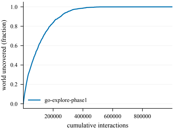
Cumulative coverage -- EnlargedChamberCount5-100@5
