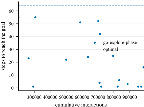
Steps to goal (train) -- EnlargedChamberCount5-100@6
