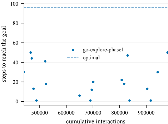
Steps to goal (train) -- EnlargedChamberCount5-100@7
