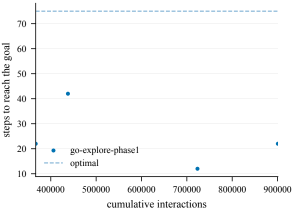
Steps to goal (train) -- EnlargedChamberCount6-120
