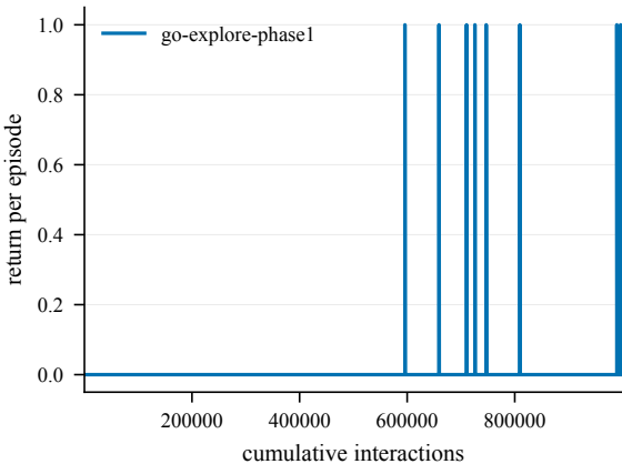
Return -- EnlargedChamberCount6-120@1
