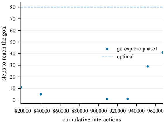
Steps to goal (train) -- EnlargedChamberCount6-120@4
