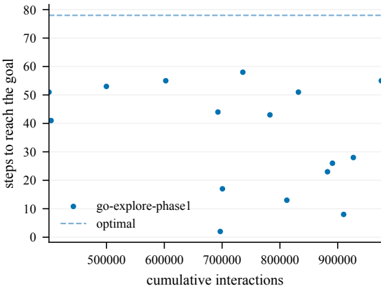
Steps to goal (train) -- EnlargedChamberCount6-120@8
