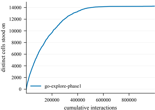
States discovered -- EnlargedChamberCount6-120@9
