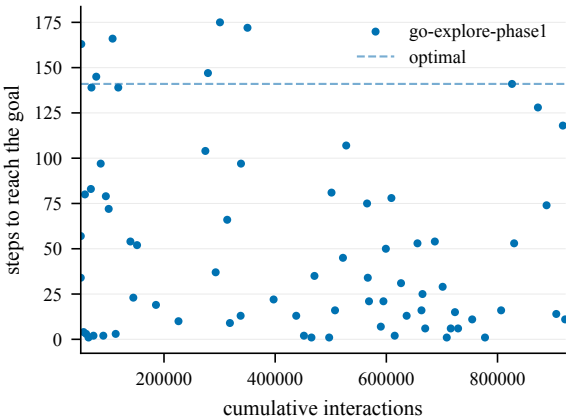
Steps to goal (train) -- EpicChase1-60@1
