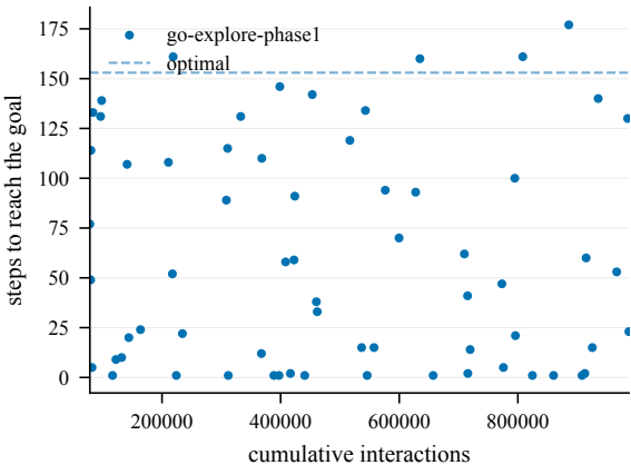
Steps to goal (train) -- EpicChase1-60@7
