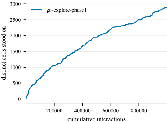
States discovered -- EpicChase12-150@1
