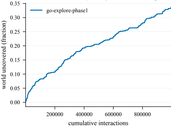
Cumulative coverage -- EpicChase12-150@11
