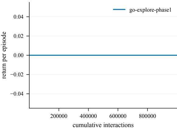
Return -- EpicChase12-150@14
