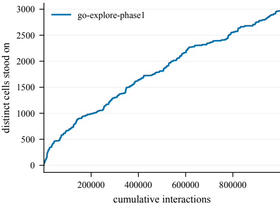
States discovered -- EpicChase12-150@14
