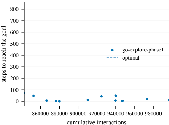
Steps to goal (train) -- EpicChase12-150@17
