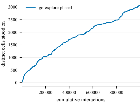
States discovered -- EpicChase12-150@18
