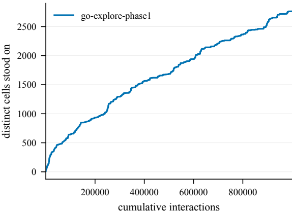
States discovered -- EpicChase12-150@19
