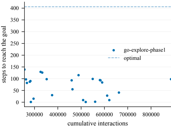
Steps to goal (train) -- EpicChase12-150@2
