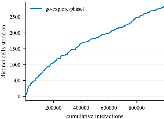
States discovered -- EpicChase12-150@2
