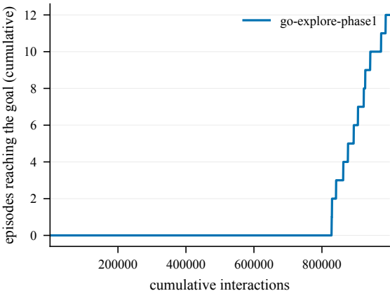
Goal reached -- EpicChase12-150@21
