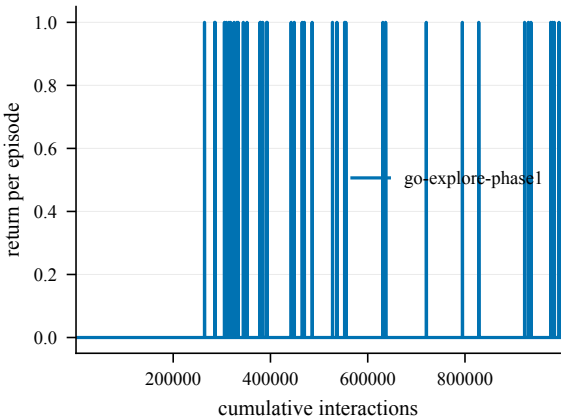
Return -- EpicChase12-150@23
