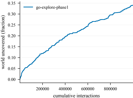
Cumulative coverage -- EpicChase12-150@25
