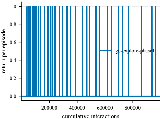
Return -- EpicChase12-150@27
