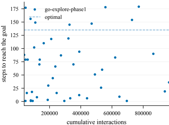
Steps to goal (train) -- EpicChase12-150@27
