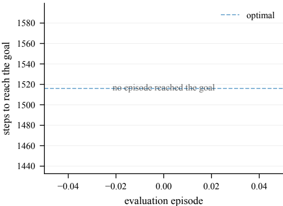
Steps to goal (eval) -- EpicChase12-150@28
