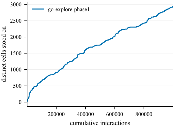
States discovered -- EpicChase12-150@28
