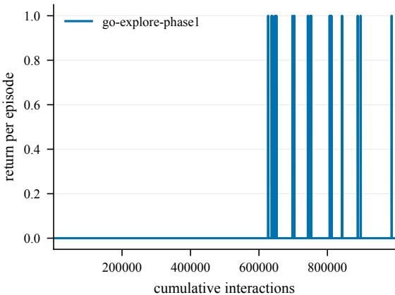
Return -- EpicChase12-150@29
