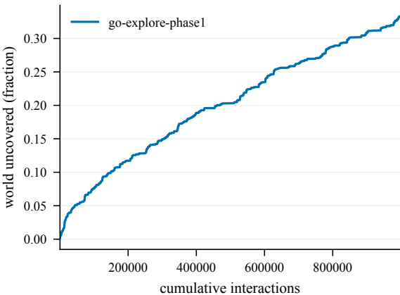
Cumulative coverage -- EpicChase12-150@3
