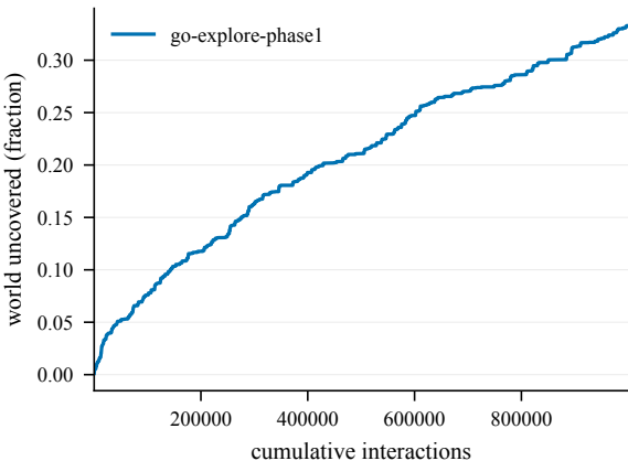
Cumulative coverage -- EpicChase12-150@4
