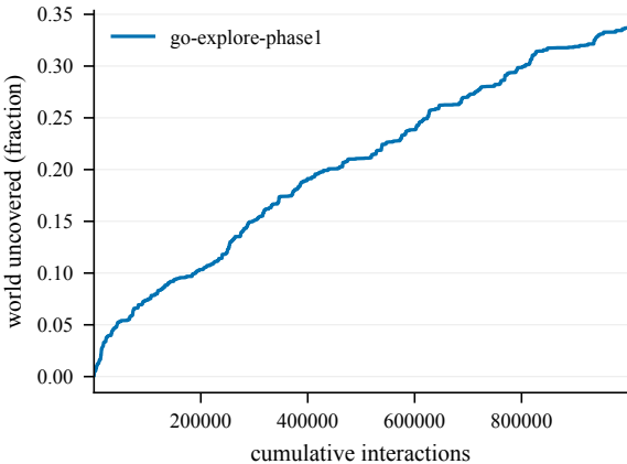
Cumulative coverage -- EpicChase12-150@5
