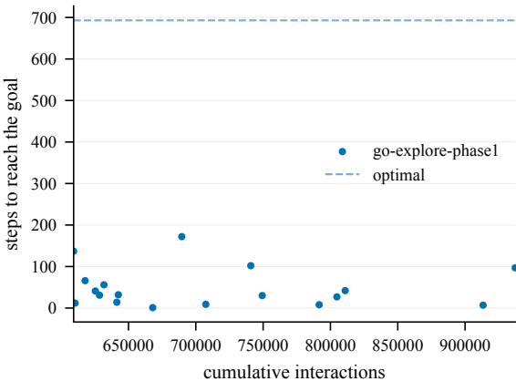
Steps to goal (train) -- EpicChase12-150@5
