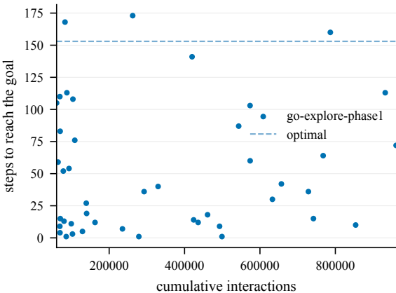
Steps to goal (train) -- EpicChase12-150@7
