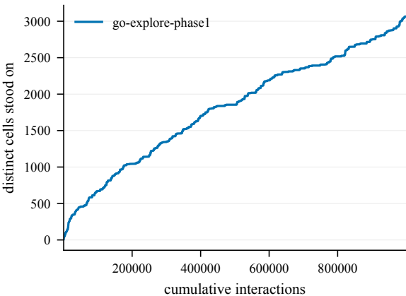
States discovered -- EpicChase12-150@9
