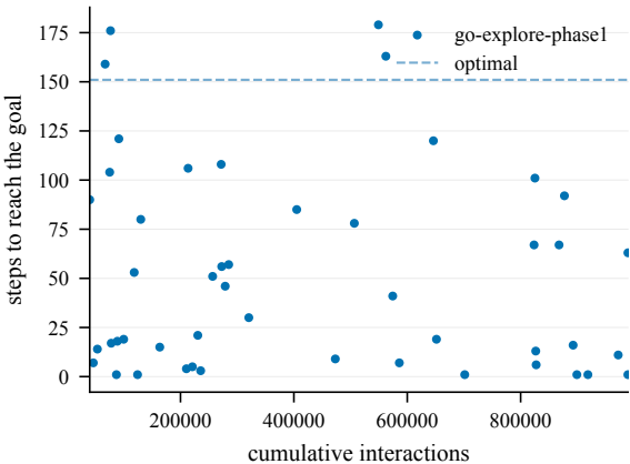
Steps to goal (train) -- EpicChase2-70
