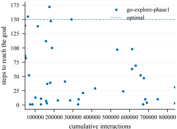
Steps to goal (train) -- EpicChase2-70@2
