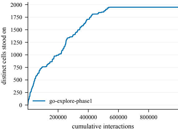
States discovered -- EpicChase2-70@2
