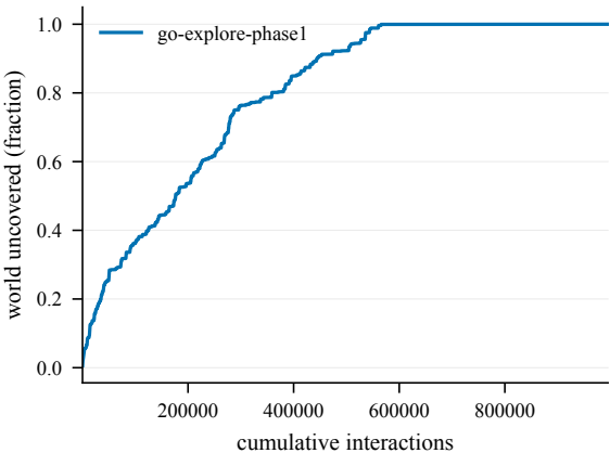
Cumulative coverage -- EpicChase2-70@7
