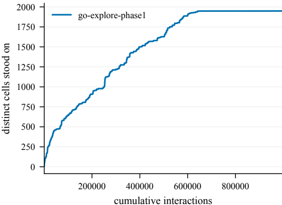
States discovered -- EpicChase2-70@8
