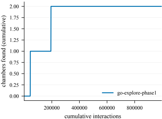
Chambers -- EpicChase2-70@9
