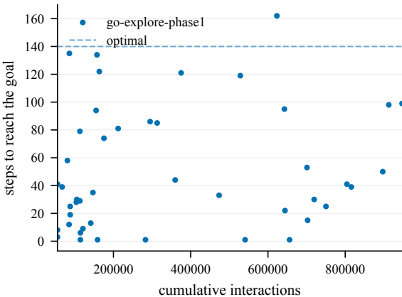
Steps to goal (train) -- EpicChase2-70@9
