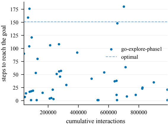
Steps to goal (train) -- EpicChase3-70
