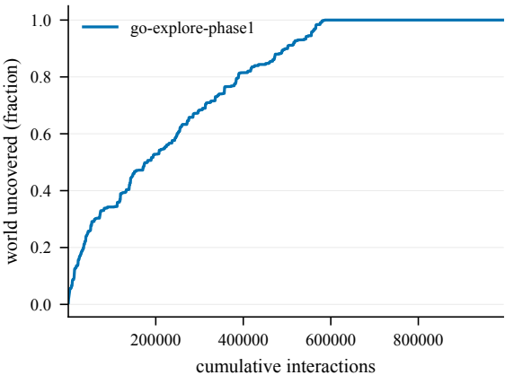
Cumulative coverage -- EpicChase3-70@1
