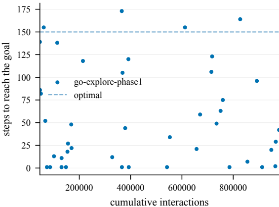
Steps to goal (train) -- EpicChase3-70@3
