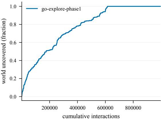
Cumulative coverage -- EpicChase3-70@4
