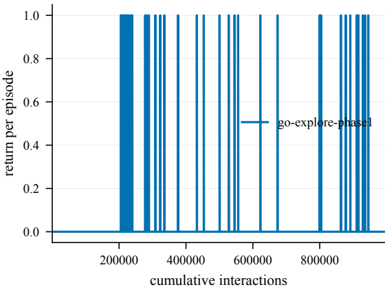
Return -- EpicChase3-70@5
