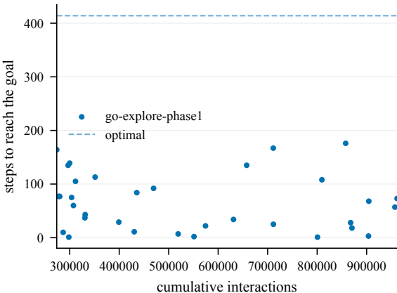
Steps to goal (train) -- EpicChase3-70@6
