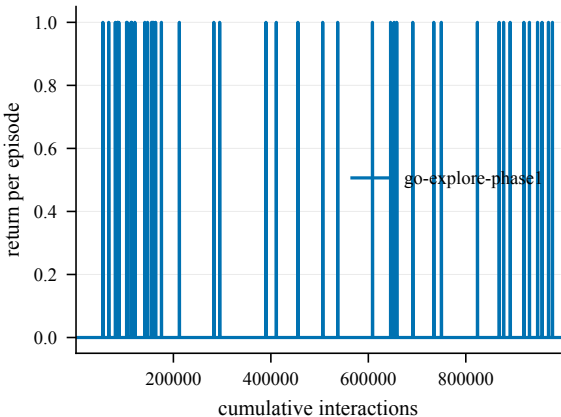
Return -- EpicChase3-70@9
