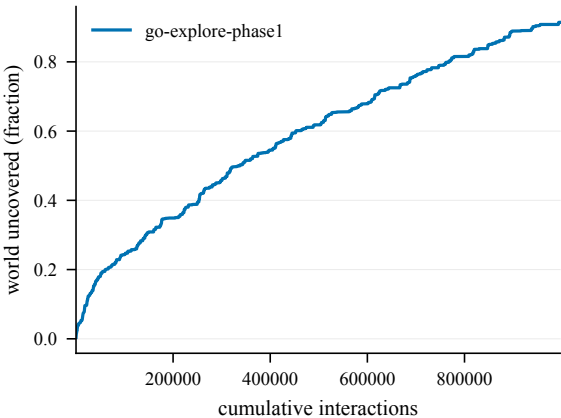
Cumulative coverage -- EpicChase4-90@5
