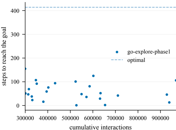
Steps to goal (train) -- EpicChase4-90@5
