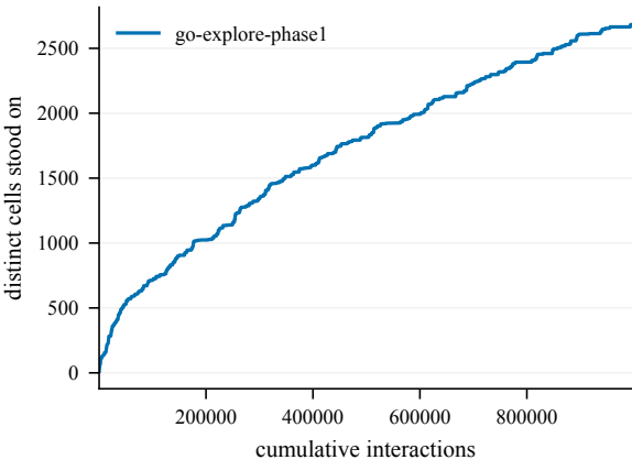
States discovered -- EpicChase4-90@5
